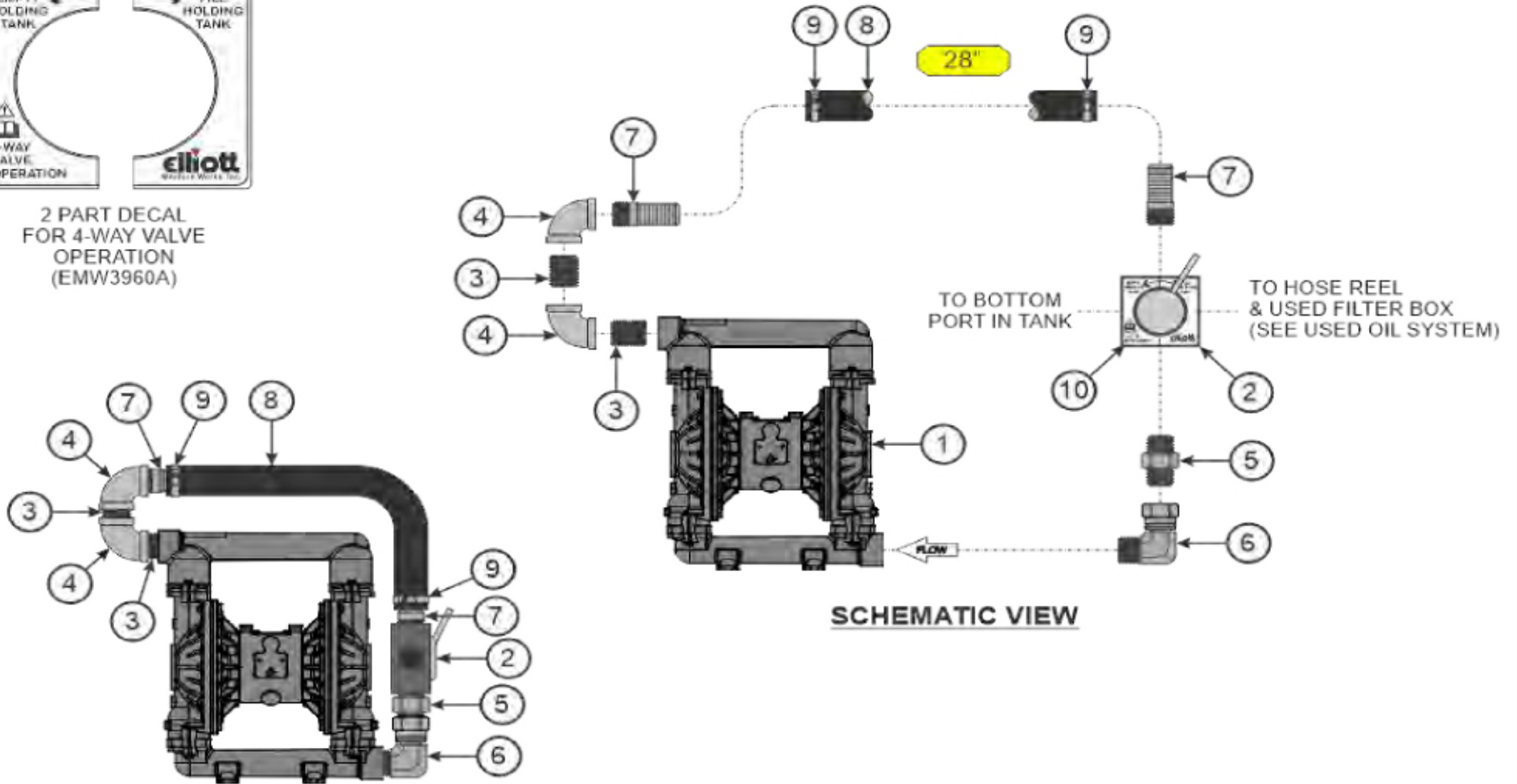
ASSEMBLED VIEW
