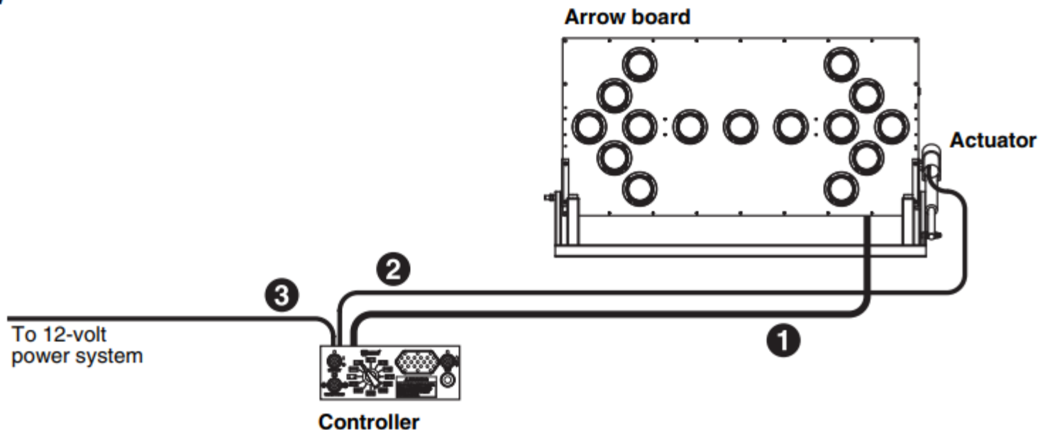
Figure 4-2. System wiring for wired controllers
