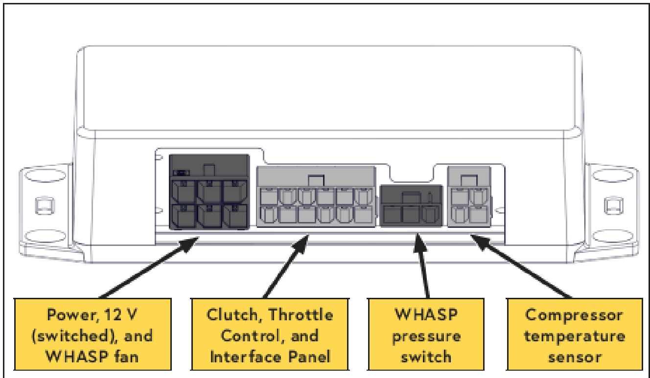
Figure 51 — Control Module
