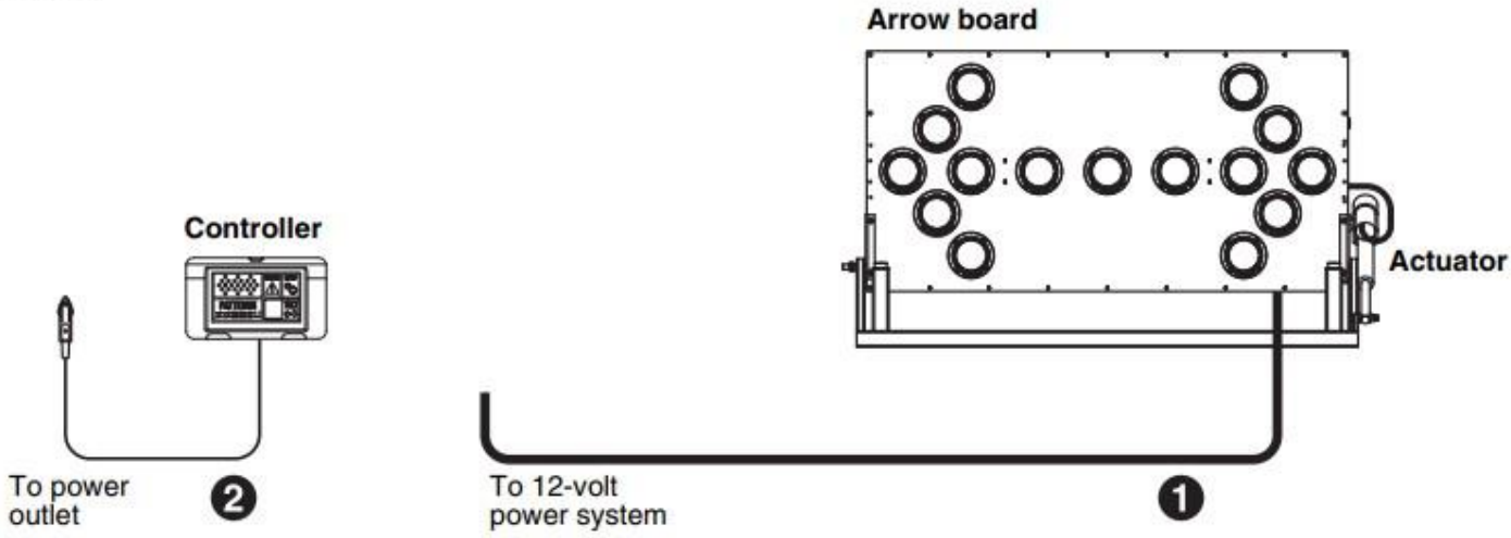
Figure 4-3. System wiring for wireless controllers
